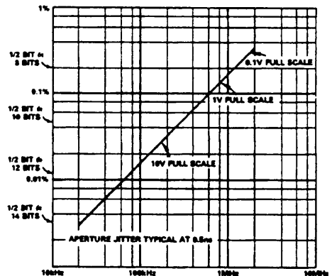
Figure 11. Aperture Jitter Error vs. Frequency
