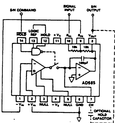
Figure 5. DIP Pin Configuration
