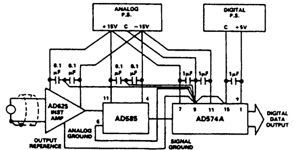
Figure 15. Basic Grounding Practice
