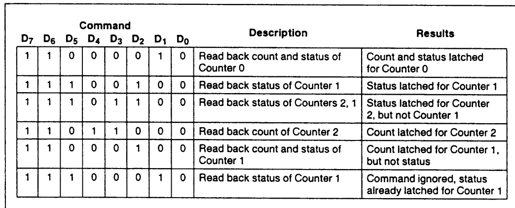
Figure 13. Read-Back Command Example
