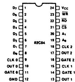
Figure 2. 82C54 Pinout
